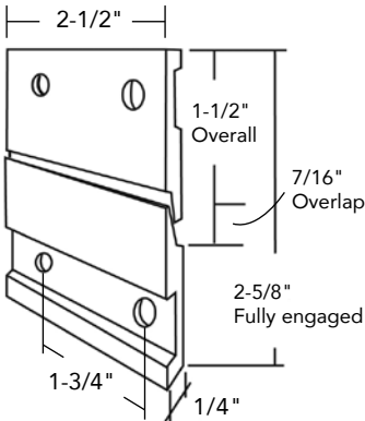
HC2 Clips - 2-1/2" width Sold per pair
